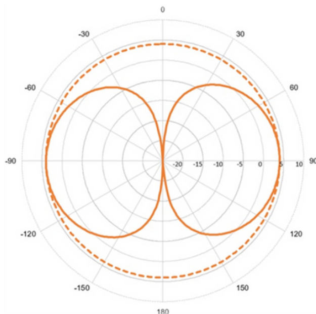
DT-11 Radiation Pattern 350-470 MHz
