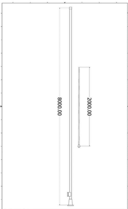
FIGURE 1: Antenna Dimensions
