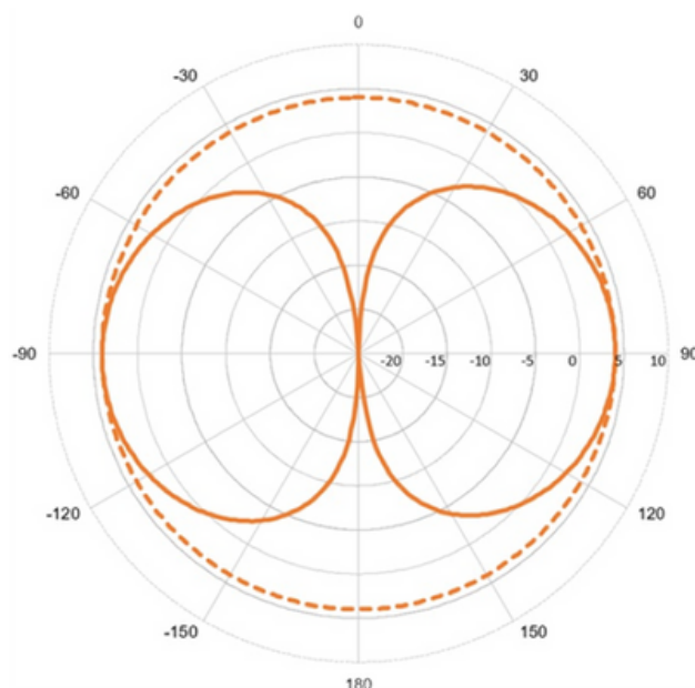
DT-11 Radiation Pattern 150-170 MHz
